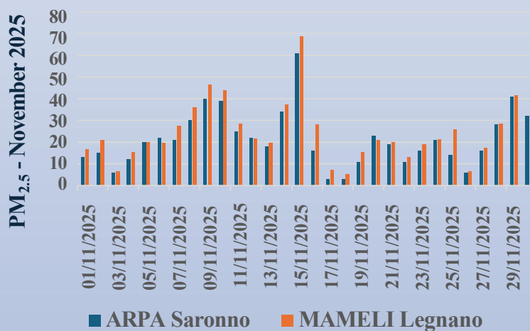
PM 2.5 - November 2025
