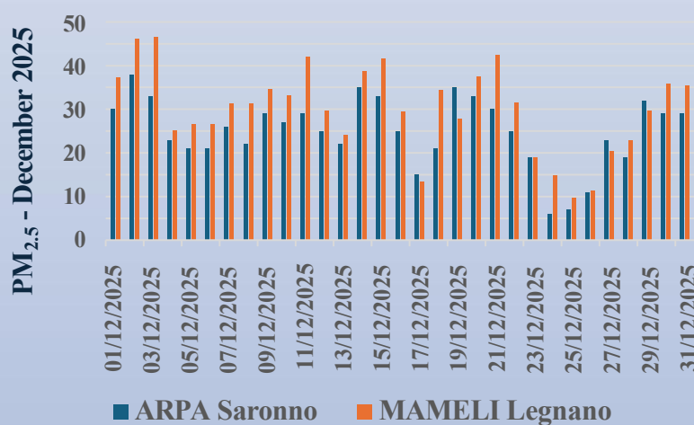
PM 2.5 - December 2025
